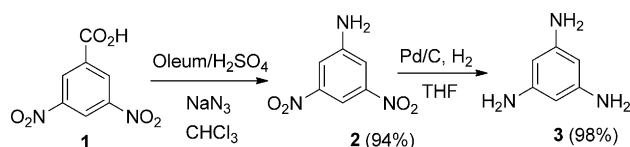
Scheme 1. Synthesis of 1,3,5-triaminobenzene.
