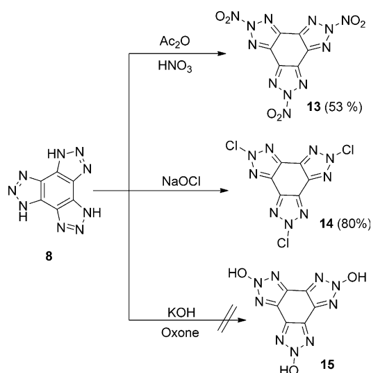
Scheme 4. N-Functionalization of tris(triazolo)benzene.
